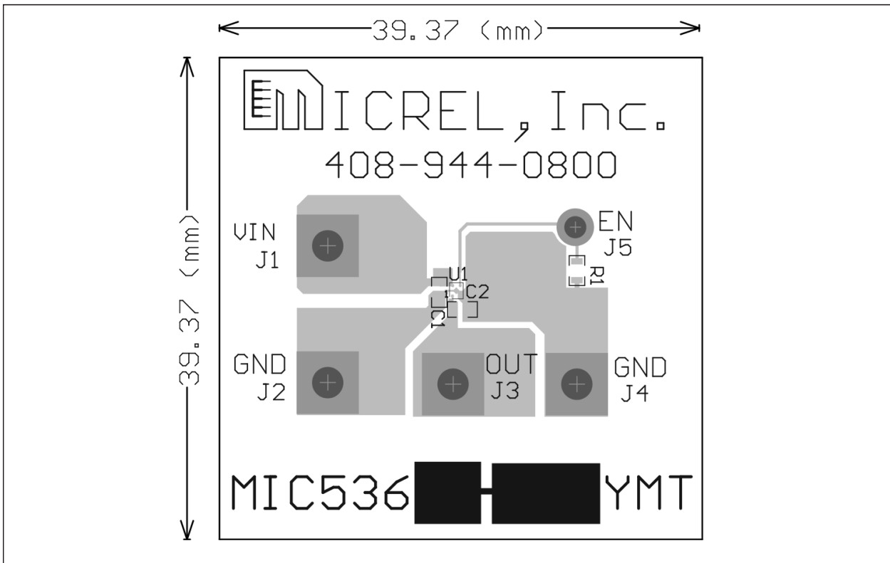
FIGURE 6-1: Top Layer.
