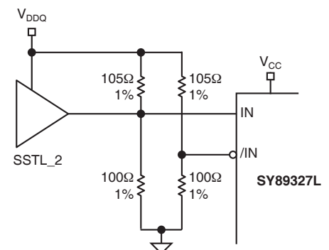
Figure 12. SSTL_2
