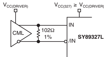
Figure 5. CML-DC Coupled
