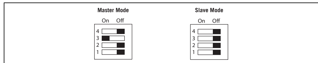
FIGURE 4-2: SETTING DIPSWITCH 2 FOR DEPLOYMENT
