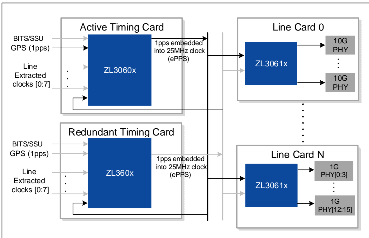
Figure 2. System with timing redundancy
