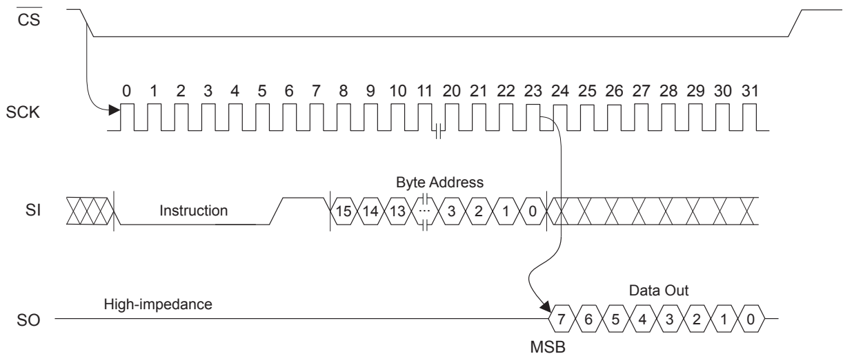
Figure 7-6. Read Timing
