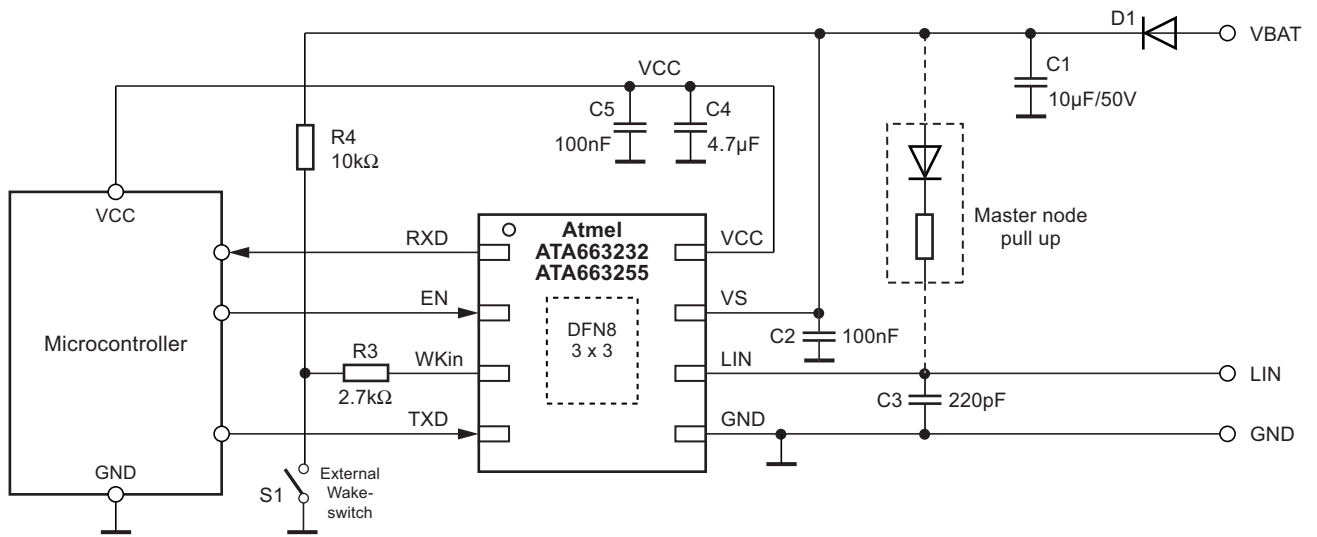
Figure 4-3. Typical Application Circuit Atmel ATA663232/55
