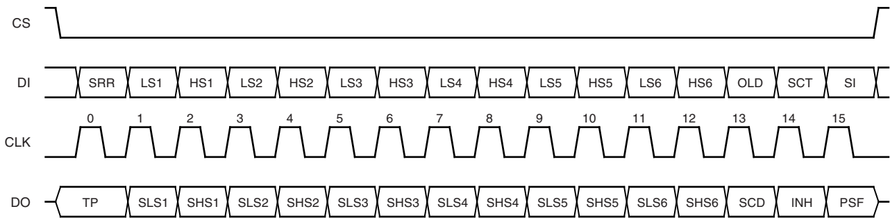
Figure 3-1. Data Transfer
